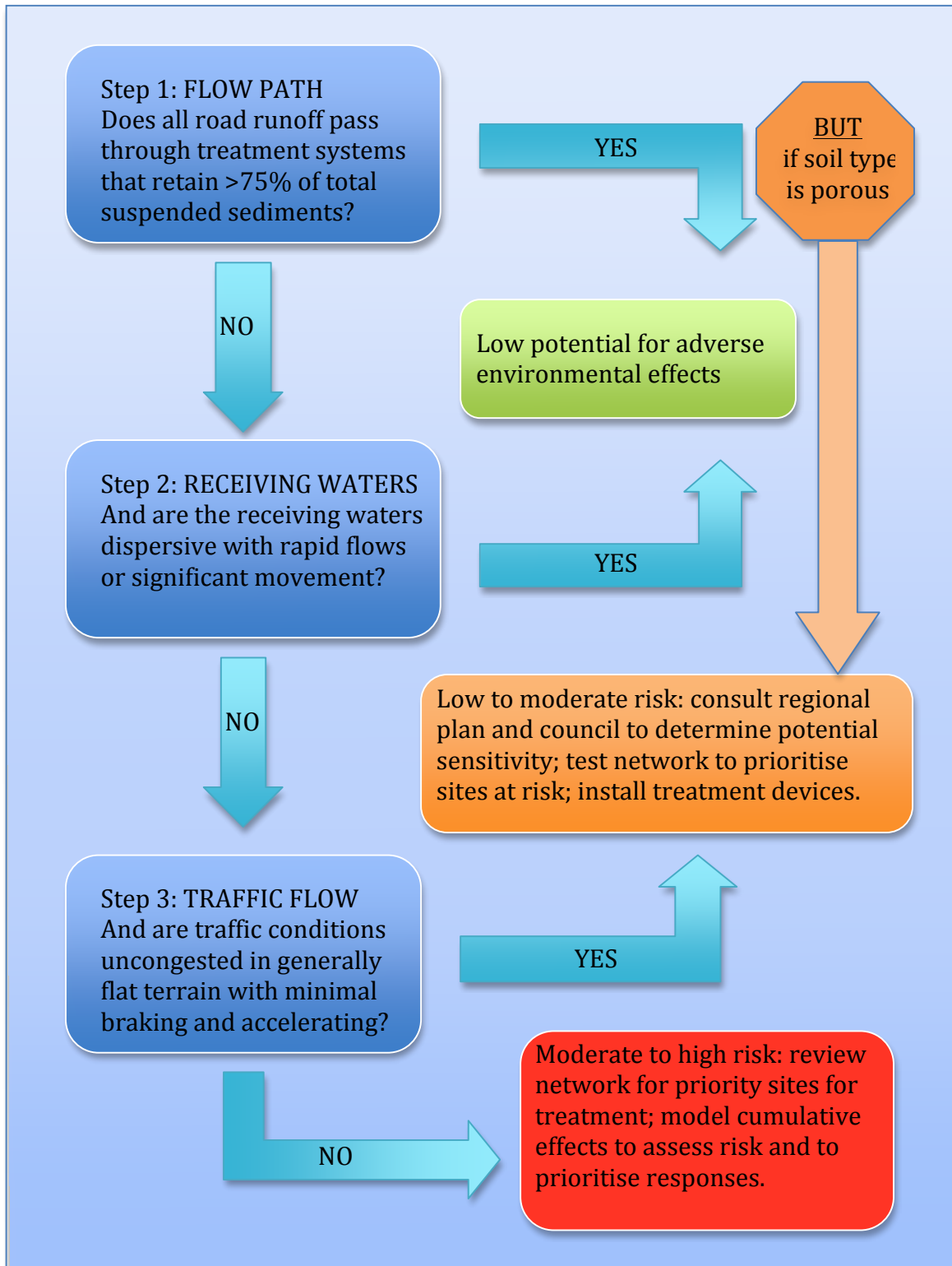
Simplified flowchart for assessing environmental risk from road runoff
